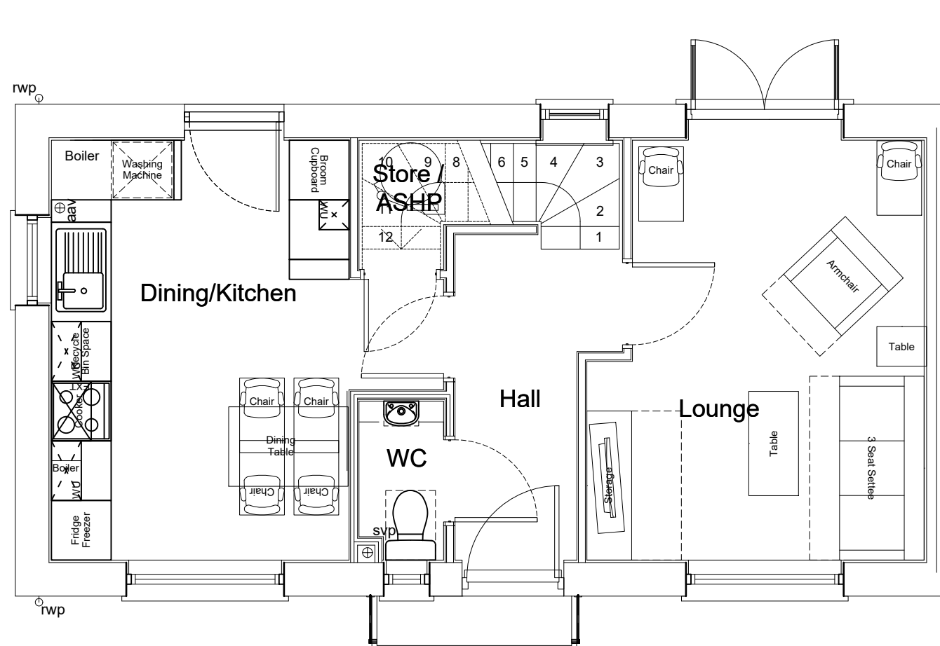
2 BED HOUSE TYPICAL GROUND FLOOR PLAN
