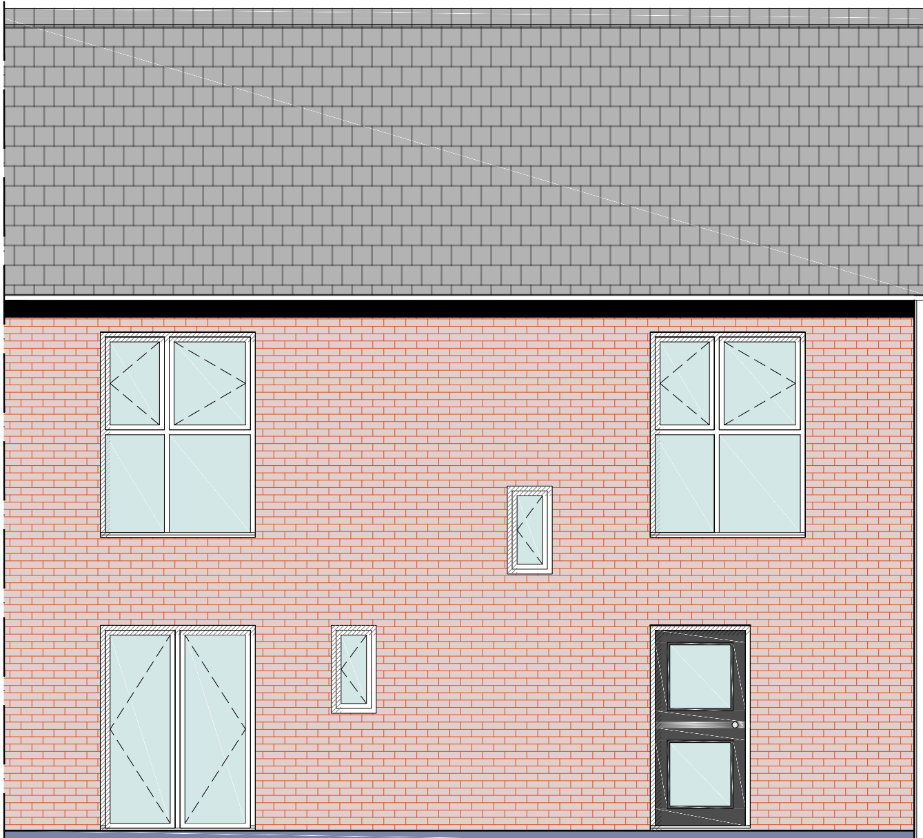
2 BED HOUSE TYPICAL REAR ELEVATION
